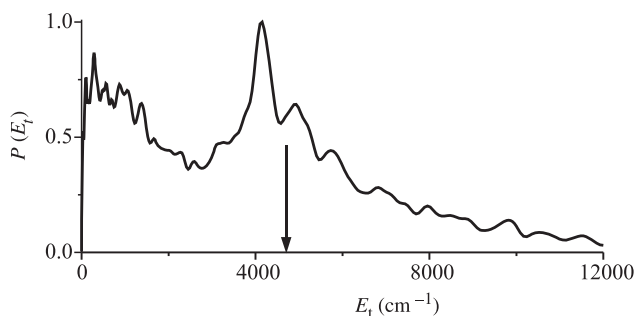
Figure 4. Photofragments c.m. kinetic energy distribution P(E_i) obtained in the photodissociation of the \text{CH}_2\text{Cl} radical at 266 nm. The distribution was derived from an image recorded by monitoring the \text{Cl}(^2P_{3/2}) fragment by 2+1 REMPI. The arrow indicates the maximum allowed kinetic energy release according to the thermochemistry for radicals in their ground vibrational state. The bands at higher kinetic energies, separated by \sim 800\text{ cm}^{-1} , correspond to excited vibrational levels of the parent \text{CH}_2\text{Cl} radical.
