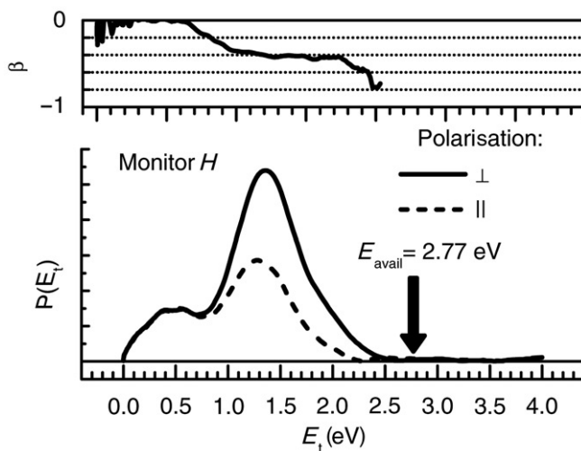
Figure 15. Photofragment c.m. kinetic energy distribution P(E_t) of \text{CH}_3\text{CHOH} obtained by monitoring H photofragments following excitation to the 3s state at 31,250\text{ cm}^{-1} ( 3.87\text{ eV} ). The arrow indicates the available energy. The recoil anisotropy parameter \beta is plotted as a function of E_t in the top panel. Reprinted with permission from [122]. Copyright (2006), American Chemical Society.
