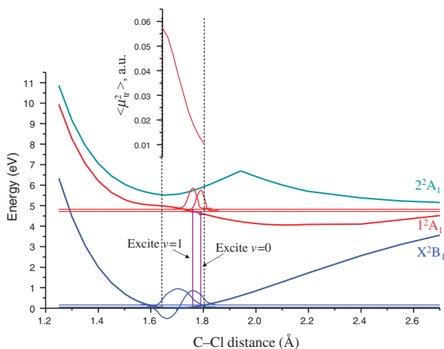
Figure 7. [Colour online] Efficient ‘hot band’ excitation in \text{CH}_2\text{Cl} results from a combination of nuclear Franck–Condon factors and changes in transition dipole moment with C–Cl bond distance. When excitation takes place from the ground vibrational state of \text{CH}_2\text{Cl} , both the Franck–Condon factor and the electronic transition moment, which is depicted at the top of the figure, are small. When a higher vibrational level is excited at the same energy, the Franck–Condon factor is larger and excitation takes place at shorter C–Cl distances, where the transition moment is larger as well. See the text for details.
