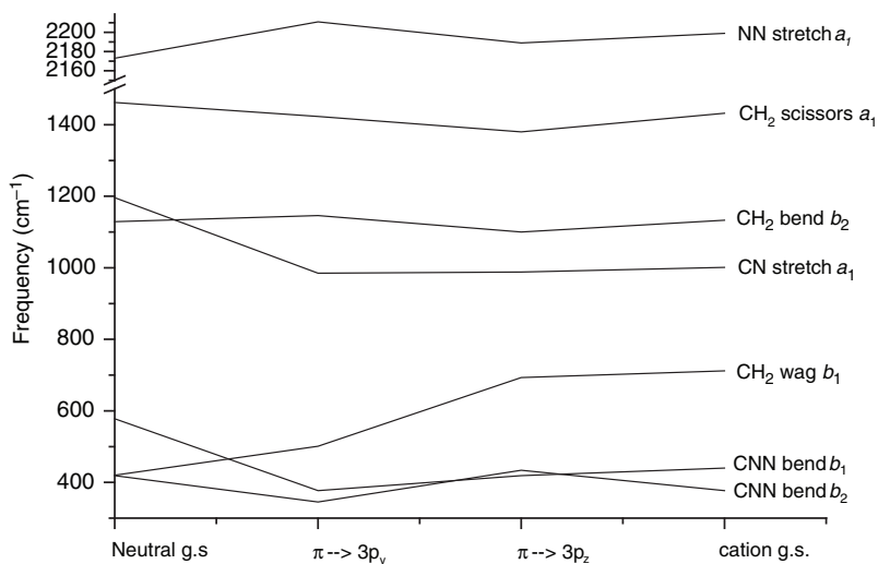
Figure 10. Harmonic vibrational frequencies of the neutral and cation ground states of diazomethane, and of the {}^2A_2 ( 3p_y ) and {}^2B_1 ( 3p_z ) excited Rydberg states. Reprinted with permission from [101]. Copyright (2007), American Chemical Society.
