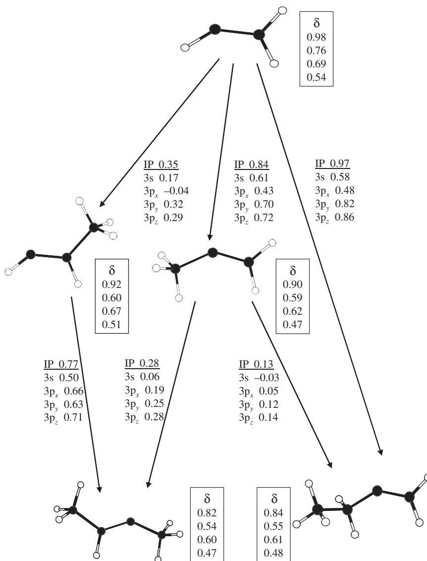
Figure 9. Quantum defects \delta for the nl_m \leftarrow n Rydberg states of vinyl and substituted vinyl radicals. Arrows connect species that differ by a single substitution of a hydrogen by a methyl or ethyl group. Next to the arrows, the differences in IEs, and in the excitation energies for the connected species are shown. The boxes show the corresponding changes in \delta , written in the order (from top to bottom): 3s, 3p x , 3p y and 3p z . Reprinted with permission from [12]. Copyright (2006), American Chemical Society.
