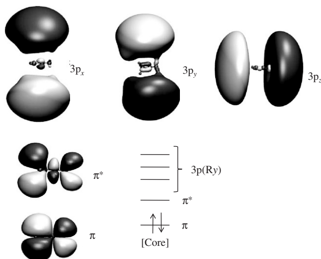
Figure 2. MOs of diazomethane. Low-lying states are derived by excitations from the HOMO to the valence \pi^* -like orbital and three diffuse 3p-like orbitals. The lowest valence state derived from excitation to the \pi_\sigma^* orbital does not interact with the Rydberg states and is not shown.
