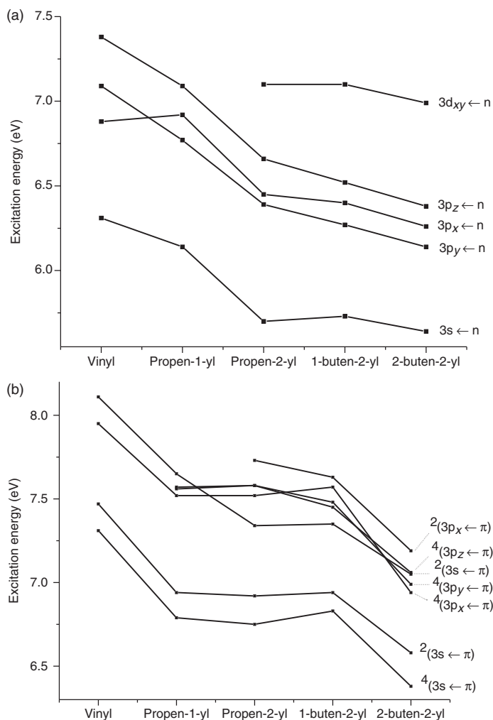
Figure 3. Changes in the nl_m \leftarrow n (upper panel) and nl_m \leftarrow \pi vertical excitation energies in vinyl and substituted vinyl radicals. Reprinted with permission from [12]. Copyright (2006), American Chemical Society.
