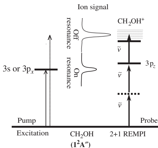
Figure 12. Schematic representation of the depletion method used to identify electronic transitions to dissociative states of jet cooled \text{CH}_2\text{OH} radicals. When the pump frequency matches an absorption band in the transition to the 3s or 3p_x states, the population of the ground state of the radical is reduced. The ground state population is monitored via a 2+1 REMPI probe signal centered on the origin band of the 2^2A''(3p_z) \leftarrow 1^2A'' transition. The signal decreases whenever absorption to the 3s or 3p_x state precedes 3p_z excitation.
