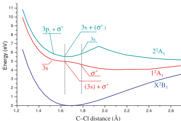
Figure 6. [Colour online] Changes in character and mixing in the 1^2A_1 and 2^2A_1 electronic states of \text{CH}_2\text{Cl} along the C–Cl stretch coordinate. The two vertical lines indicate the Franck–Condon region.
