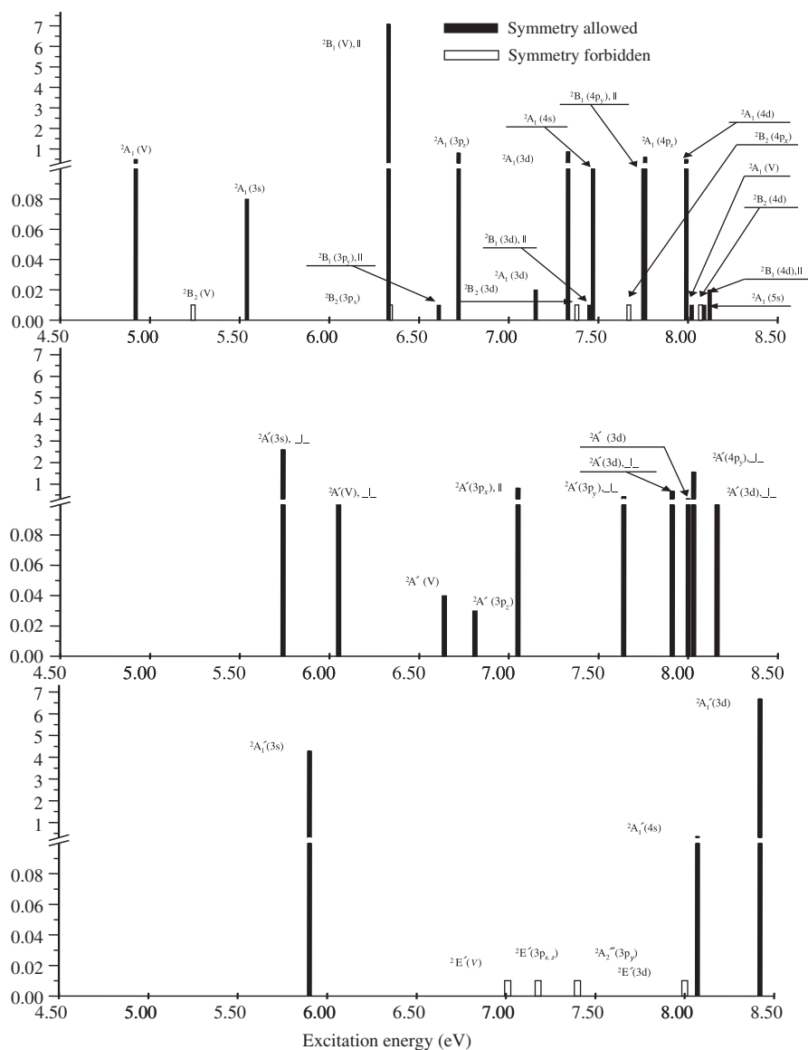
Figure 8. Vertical excitation energies for CH 2 Cl (top panel), CH 2 F (middle panel), and CH 3 (bottom panel). Intensities of the transitions are proportional to the oscillator strengths (no Franck–Condon factors are taken into account). Empty bars show positions of forbidden transitions, i.e. those for which the oscillator strength is zero due to symmetry. Transitions are defined as parallel when the transition dipole moment is parallel to the CX bond, and perpendicular otherwise. Reprinted with permission from [21]. Copyright (2001), American Institute of Physics.
