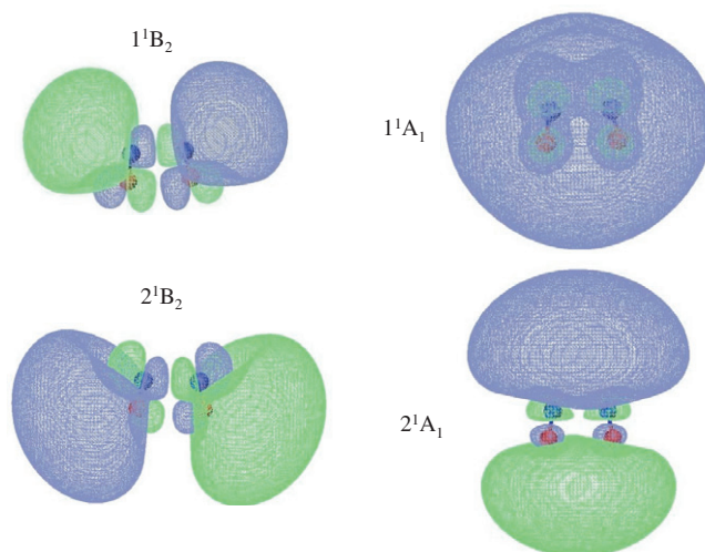
Figure 1. Dyson orbitals corresponding to the two B_2 (left) and two A_1 states of (NO)_2 . (Note: the numbering of the states is not spectroscopic and is only used to distinguish between the states, e.g. 1A_1 state is not the lowest A_1 state of the dimer; rather, it is the lowest of the two A_1 Rydberg states considered in this example). The B_2 states are of mixed Rydberg–valence character, whereas the A_1 states are predominantly Rydberg. Note the similarity between the respective Dyson MOs and the hydrogen-atom like orbitals.
